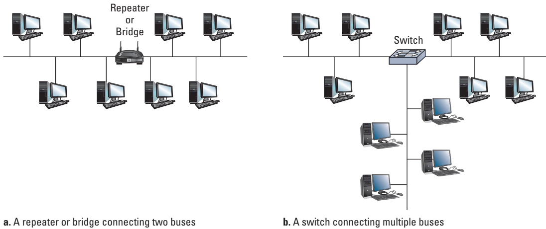
Figure 4.4 Building a large bus network from smaller ones
